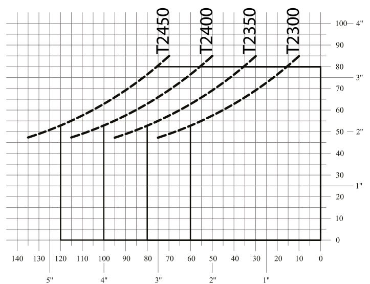
Cutting diagram
